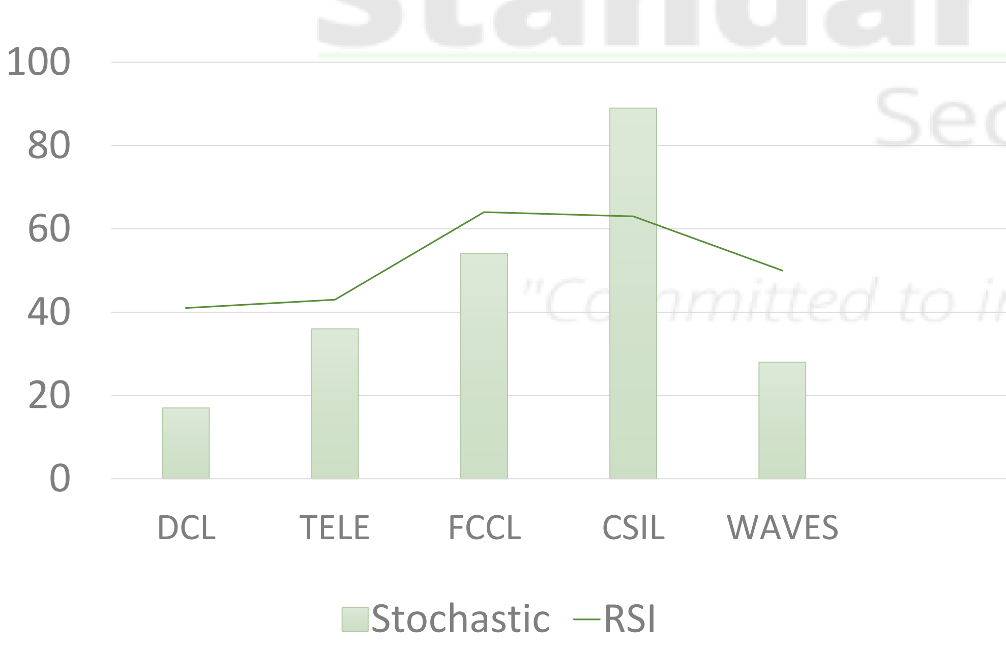
RSI and Stochastic Indicators
